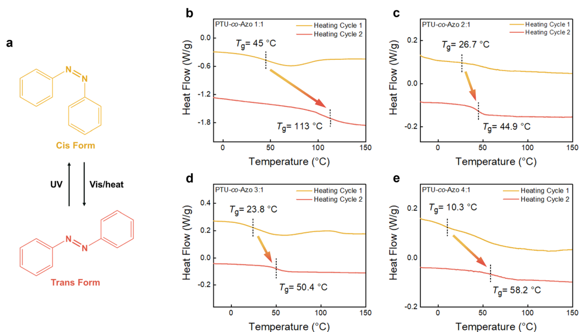
Fig. 4 (a) Cis – trans isomerization of the azobenzene groups in PTUEG 3 -co-Azo copolymer films under UV and visible light irradiations. (b)–(e) Differential scanning calorimetry (DSC) thermograms of PTUEG 3 -co-Azo copolymers with TUEG-DA:Azo-DA ratios of (b) 1:1, (c) 2:1, (d) 3:1, and (e) 4:1, showing glass transition temperatures ( T_g ) during first and second heating cycles. The first heating cycle curves have been vertically offset for clarity.
