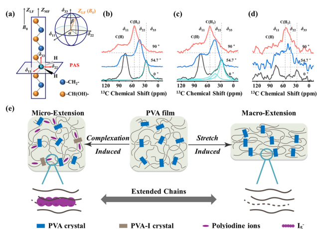
Fig. 15 (a) Schematic of the orientation of the chain axis and CSA tensors of CH 2 (when the stretching direction of the PVA samples was placed at 01 orientation with respect to the B 0 field). (b–d) Static three-phase 13 C CP spectra measured using the static probe of three phases for the oriented-0 M sample (0 M–5 M) with different orientations relative to the B 0 field. (e) Schematic of the effect of macroscopic extension and microscopic complexation on PVA chains. Reprinted with permission from ref. 136; copyright 2022, the Royal Society of Chemistry.
