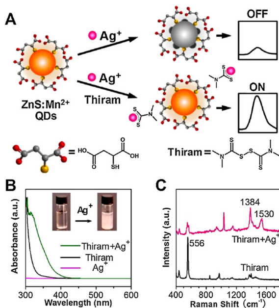
Fig. 21 (A) The sensing mechanism for the detection of thiram. (B) UV-vis absorption spectra of Ag(I), thiram, and Ag–thiram complex (inset: colloidal suspension of the complex). (C) The Raman spectra of thiram and Ag–thiram complex. Reprinted with permission from ref. 200. Copyright 2017 Elsevier.
