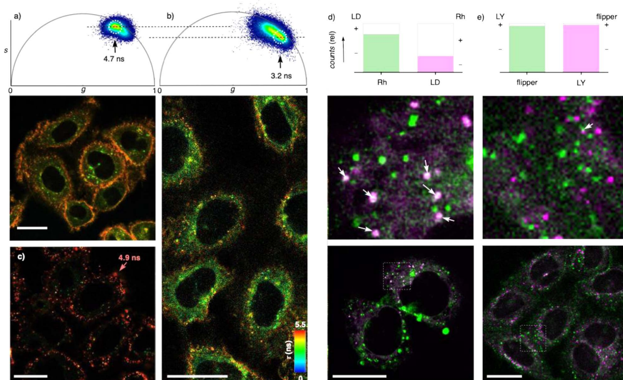
Fig. 4 (a–c) FLIM images of HK cells incubated for 2 h with (a) flipper 12 and (b) DSP 5 C LUVs 5 and (c) DSPC LUVs 6, both with 1% 12, with phasor plots 84 for fit-free lifetime analysis for (a) and (b), top). (d) CLSM image of HK cells incubated with DSP 5 C LUVs 5 containing 1% Rh-PPPE (green) and lipid droplet tracker (LD, magenta, bottom), with zoom (middle) and relative counts of LD tracker without (magenta) and with co-localization with Rh (white, top right), and Rh without (green) and with co-localization with LD tracker (white, top left). (e) CLSM image of HK cells incubated with DSP 5 C LUVs 5 containing 1% flipper 12 (green) and LysoTracker (LY, magenta, bottom), with zoom (middle) and relative counts of LY tracker without (magenta) and with co-localization with flipper (white) and flipper without (green) and with co-localization with LY tracker (white, top); scale bars = 20 \mu m.
