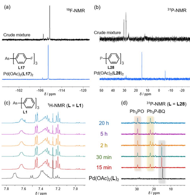
Fig. 8 NMR spectra of the \text{Pd}(\text{OAc}) complexes and reaction mixtures after the catalytic reactions using (a) L17 ( ^{19}\text{F} -NMR, 376 MHz) and (b) L28 ( ^{31}\text{P} -NMR, 162 MHz) in EtOAc. Trace of the mixture of (c) L1 ( ^1\text{H} -NMR, 400 MHz) and (d) L28 ( ^{31}\text{P} -NMR, 162 MHz) (0.2 eq.), BQ (1 eq.), and AcOH (5 eq.) in \text{CDCl}_3 .
