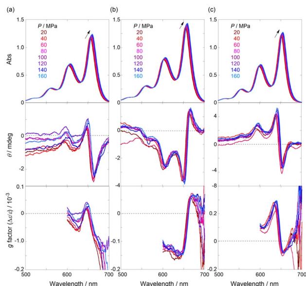
Fig. 4 Pressure-dependent UV/vis absorption (top), CD (middle), and anisotropy ( g ) factor ( =\Delta\epsilon/\epsilon ) (bottom) spectra of (a) (R,R) -Pc-EE-Pc (144 \mu M), (b) (S,S) -Pc-CE-Pc (142 \mu M), and (c) (R,R) -Pc-CA-Pc (136 \mu M) in toluene at room temperature at 20, 40, 60, 80, 100, 120, 140, and 160 MPa, measured in a high-pressure cell. The g factor profiles <600 nm were omitted due to the baseline noises.
