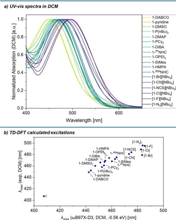
Fig. 6 (a) Normalised CT absorption bands of donor adducts in DCM. (b) Calculated ( \omega B97X-D3/def2-TZVPP/SMD(DCM)//r 2 SCAN-3c) vs. experimentally observed absorption maxima for 1 and donor complexes 1-X /[ 1-X ] − . Calculated absorption wavelengths were redshifted by 0.56 eV.
