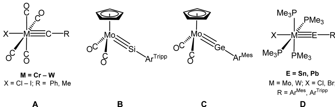
Fig. 1 First reported complexes featuring metal–tetrel triple bonds; \text{Ar}^{\text{Tripp}} = \text{C}_6\text{H}_3\text{-}2,6\text{-Tripp}_2 , \text{Tripp} = 2,4,6\text{-triisopropylphenyl} ; \text{Ar}^{\text{Mes}} = \text{C}_6\text{H}_3\text{-}2,6\text{-Mes}_2 , \text{Mes} = 2,4,6\text{-trimethylphenyl} .
