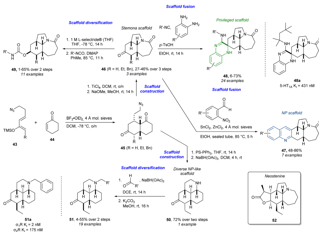
Scheme 3 Synthesis of stepona-inspired compounds and identification of 2-HT 1A ligand 48a and \sigma_1 R and \sigma_2 R ligand 51a . 85–87 L-selectride® = lithium tri- sec -butylborohydride, PS-PPh 3 = polystyrene bound triphenyl phosphine.
