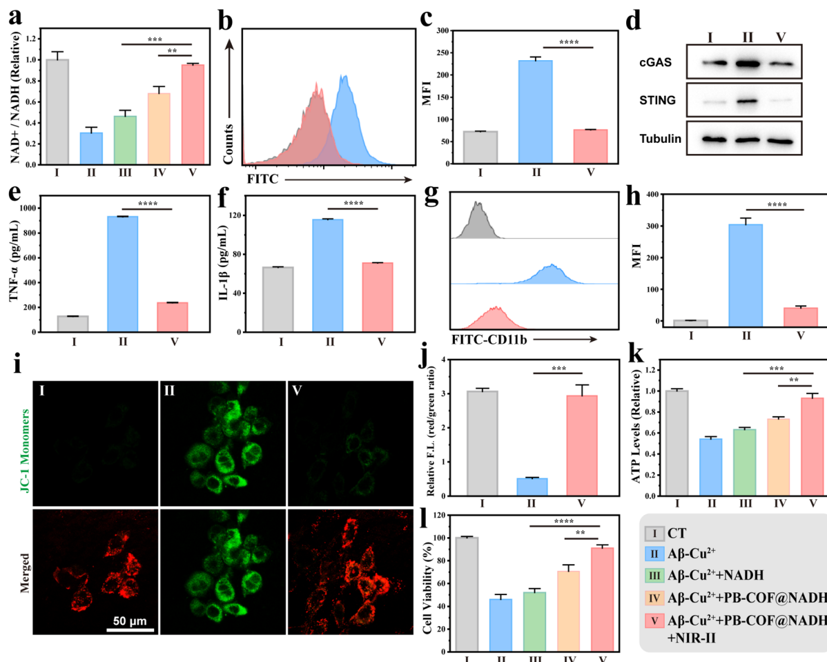
Fig. 4 (a) \text{NAD}^+/\text{NADH} ratio of HT22 cells incubated with \text{A}\beta\text{42-Cu}^{2+} following various treatments. (b and c) Flow cytometry (b) and corresponding quantitative analysis of intracellular ROS levels following various treatments. The fluorescence intensity of the ROS was represented by FITC-A. (d) Protein expression of cGAS and STING under different incubation conditions, as evaluated by western blot analysis. Tubulin was used as a loading control. (e and f) Quantitative analysis of (e) \text{TNF-}\alpha secretion and (f) \text{IL-1}\beta secretion after different stimulations. (g and h) Flow cytometry (g) and corresponding quantitative analysis (h) of intracellular CD11b levels. (j and i) Mitochondrial membrane potential following various treatments (i) and quantitative analysis (j). (k) Intracellular ATP levels following various treatments. (l) Cell viability of HT22 cells after various treatments. Irradiation with a 1064 nm laser ( 1.0 \text{ W}\cdot\text{cm}^{-2} ).
