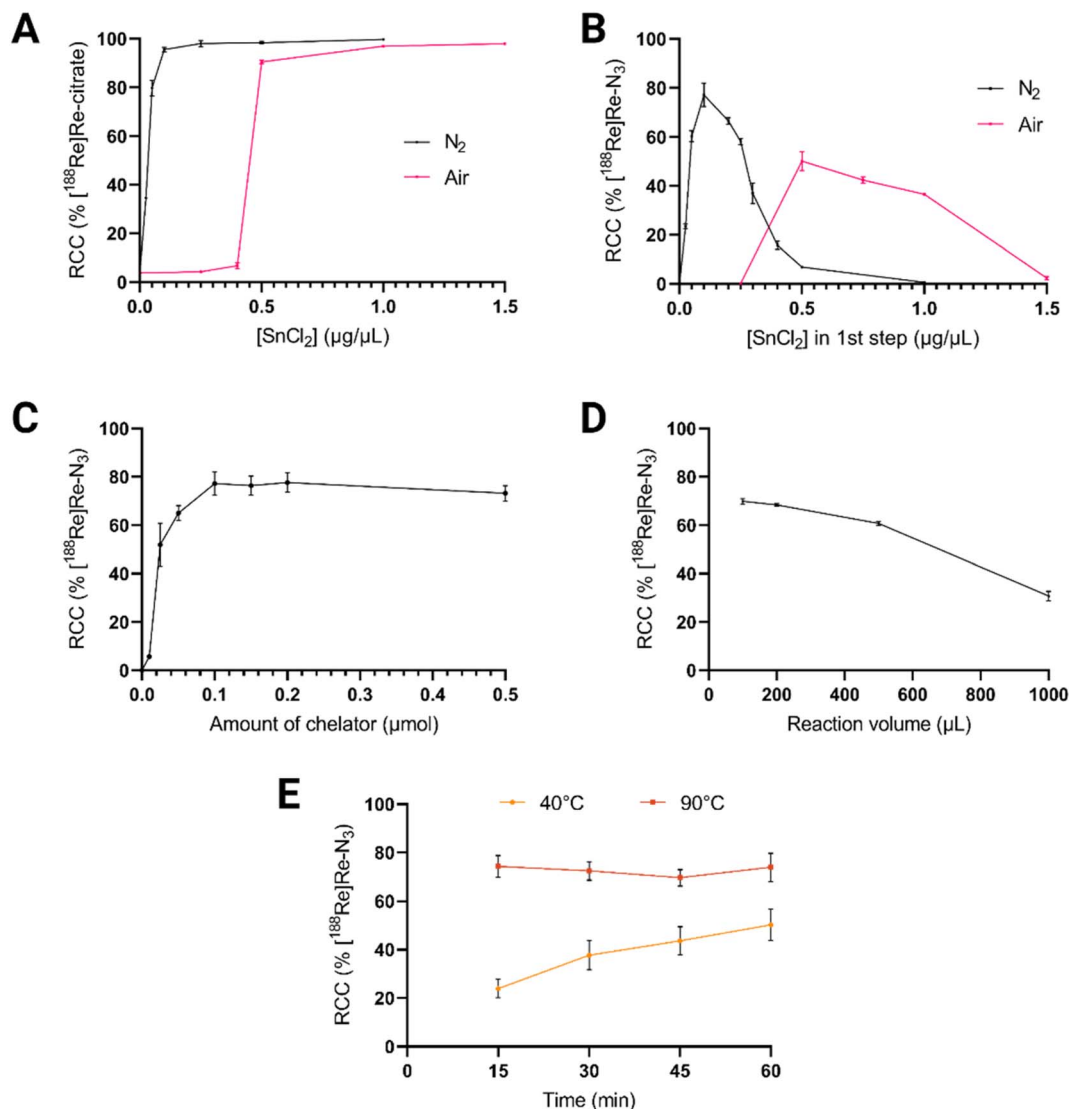
Fig. 6 Radiolabelling optimisation of [ 188 Re]ReO(N 2 S 2 -PEG 3 -N 3 ). Conditions tested: (A) influence of N 2 atmosphere; (B) SnCl 2 concentration; (C) chelator quantity; (D) reaction volume; (E) reaction temperature and time. The fixed values for each variable during the optimisations were as follows: activity (20 MBq), SnCl 2 concentration (0.1 μg μL -1 ), volume (100 μL), chelator quantity (0.1 μmol), temperature (90 °C) and time (60 min). RCC = radiochemical conversion.
