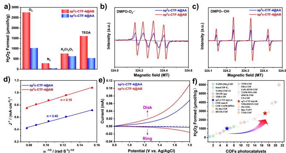
Fig. 4 (a) \text{H}_2\text{O}_2 production of \text{sp}^2\text{c-CTF-4@AA} and \text{sp}^2\text{c-CTF-4@AB} under different conditions ( \text{O}_2 , \text{N}_2 , \text{K}_2\text{Cr}_2\text{O}_7 , TEOA); (b) DMPO spin-trapping EPR spectra of \text{sp}^2\text{c-CTF-4} for measuring \text{O}_2^{\cdot-} ; (c) DMPO spin-trapping EPR spectra of \text{sp}^2\text{c-CTF-4} for measuring \cdot\text{OH} ; (d) the Koutecky–Levich plots obtained via RDE measurements in phosphate buffer (pH 7) solution with continuous \text{O}_2 purging; (e) polarization curves recorded with simultaneous detection of \text{H}_2\text{O}_2 at the ring electrode at 1600 rpm; (f) summary of photocatalytic \text{H}_2\text{O}_2 evolution rates of \text{sp}^2\text{c-CTF-4} and other COF-based photocatalysts.
