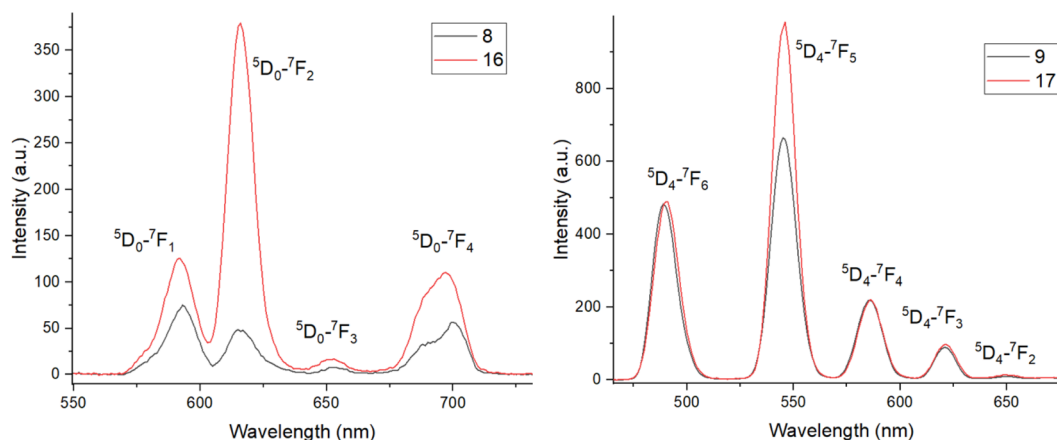
Fig. 3 Phosphorescence spectra for Eu complexes 8 and 16 (left) and Tb complexes 9 and 17 (right) (20 \mu M, slits 10 nm, PBS, 0.1 ms delay).
