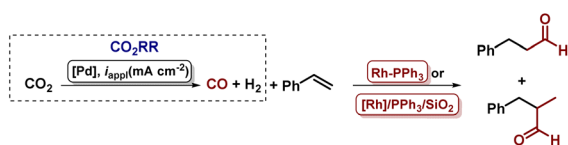
Fig. 20 Integrated electrochemical \text{CO}_2 reduction and aromatic alkenes hydroformylation with Rh catalyst in a vial-in-vial reactor.
