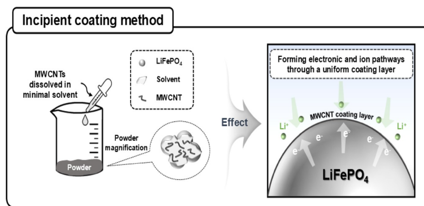
Fig. 12 Incipient coating of MWCNTs on LFP enhances electron and ion pathways. 96 Reproduced from ref. 96 with permission from the American Chemical Society, copyright 2025.
