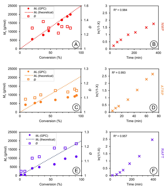
Fig. 2 RDRP reaction kinetics for DHIAMA: number average molecular weight ( M_n ) by GPC, calculated theoretical M_n , and dispersity ( D ) throughout polymerization by: (A) NMP; (C) ATRP; and (E) RAFT. Linearized monomer conversion (semi-logarithmic) during polymerization is shown by: (B) NMP; (D) ATRP; and (F) RAFT. Reaction conditions are provided in section 2.1.
