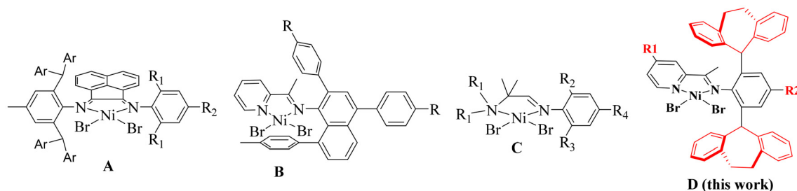
Chart 1 Typical nickel-based catalysts with diverse ligand structures in polyolefin elastomer synthesis (A–D).
