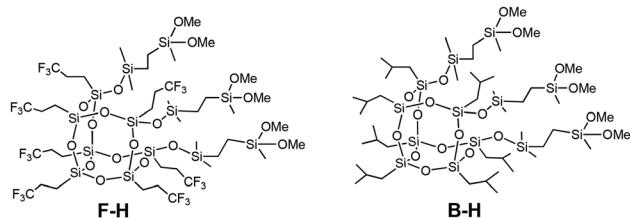
Fig. 4 Chemical structures of F-H and B-H.
