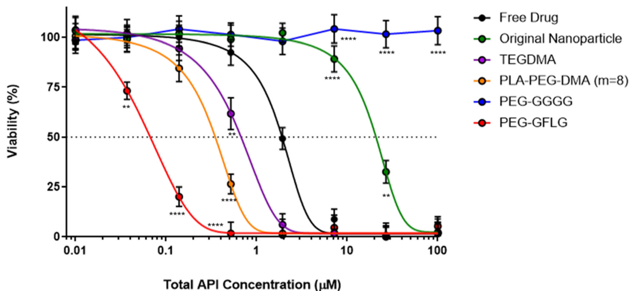
Fig. 7 In vitro efficacy of free drug compared to 5 nanoparticle formulations with paclitaxel and carboplatin loaded at the 5 : 1 ratio using OVCAR-3 cells as determined using the MTS assay. Data compares the free paclitaxel (black); the original nanoparticle composition (green); the optimized P(DEAEMA- co -CHMA)- g -PEGMA nanoparticles synthesized with varying crosslinking agents of TEGDMA (purple) and PLA-PEG-DMA m = 8 (orange); and finally the optimized P(DEAEMA- co -CHMA)- g -PEGMA nanoparticles synthesized with TEGDMA crosslinking agent and either non-CathepsinB responsively linked PEG grafts (PEG-GGGG, blue) and responsive PEG grafts (PEG-GFLG, red). Two-way ANOVA was used to test significance at each concentration of various nanoparticles compared to free drug. Significance represents ** < 0.025 , **** < 0.0001 .
