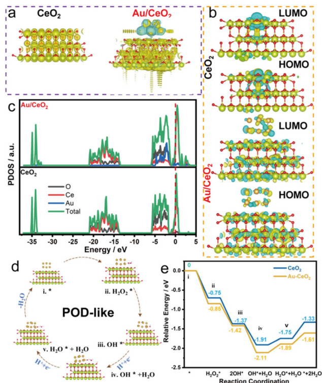
Fig. 5 (a) Charge density difference illustration of CeO 2 and Au/CeO 2 . (b) HOMO–LUMO energy levels and the interfacial diagrams of the molecular orbitals for CeO 2 and Au/CeO 2 . (c) Density of states of CeO 2 and Au/CeO 2 . (d) Proposed reaction pathways of the POD-like reaction. (e) Corresponding free energy diagrams of CeO 2 and Au/CeO 2 for the POD-like reaction.
