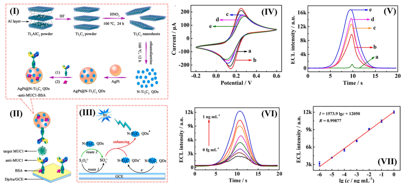
Fig. 11 Schematic representations of a MXene-QD-based ECL sensor probe for MUC1 detection. (I) The synthesis of \text{AgPt}@N\text{-MXene} QDs-anti-MUC1-BSA bioconjugates, where N-MXene QDs are combined with bimetallic AgPt nanoparticles and then conjugated with anti-MUC1 antibodies to obtain a highly selective ECL sensor probe. (II) The development of the ECL immunosensor. (III) The possible ECL mechanism of the N-MXene QDs/ \text{S}_2\text{O}_8^{2-} system; here MXene QDs act as luminophores in the presence of the co-reactant potassium persulphate, producing significantly enhanced luminescence via intermediate generation. (IV) The CV response of each modified electrode: a bare GCE (a), DpAu/GCE (b), anti-MUC1/DpAu/GCE (c), BSA/anti-MUC1/DpAu/GCE (d), and MUC1/BSA/anti-MUC1/DpAu/GCE (e), confirming the step-by-step modification of the sensor probe. (V) A comparison of ECL responses after each modification of the sensor showing the ECL intensities of (a) N- \text{Ti}_3\text{C}_2 QDs in PBS solution, (b) N- \text{Ti}_3\text{C}_2 QDs in \text{S}_2\text{O}_8^{2-} solution, (c) N- \text{Ti}_3\text{C}_2 QDs in \text{S}_2\text{O}_8^{2-} solution with Ag nanoparticles, (d) N- \text{Ti}_3\text{C}_2 QDs in \text{S}_2\text{O}_8^{2-} solution with Pt nanoparticles, and (e) N- \text{Ti}_3\text{C}_2 QDs in \text{S}_2\text{O}_8^{2-} solution with AgPt nanoparticles, which demonstrates the highest ECL response due to the synergistic effect of bimetallic AgPt nanoparticles. (VI) The ECL responses of the fabricated immunosensor to various concentrations of MUC1, highlighting the concentration-dependent increase in the ECL signal due to antigen-antibody interactions. (VII) The calibration plot of the developed sensor for MUC1 detection, representing the sensitivity and stability of the sensor probe. Reproduced with permission from ref. 242; copyright 2022, ELSEVIER.
