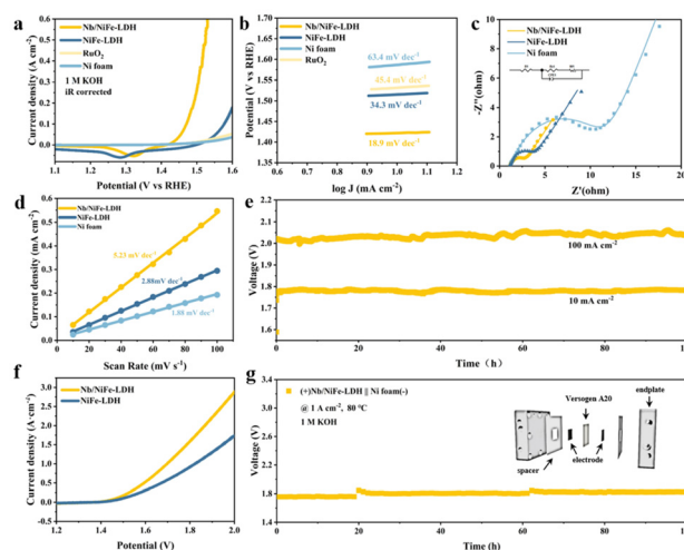
Fig. 2 (a) LSVs and (b) Tafel plots of various samples; (c) Nyquist plots of various samples; (d) plots showing the extracted C dl value to estimate the ECSA; (e) stability test of Nb/NiFe-LDH at a current density of 0.01 A cm -2 and 0.1 A cm -2 ; (f) LSVs of the AEM electrolyzer using Nb/NiFe-LDH||Ni foam and NiFe-LDH||Ni foam in 1.0 M KOH; and (g) durability test of the AEM electrolyzer using Nb/NiFe-LDH||Ni foam at 1.0 A cm -2 in 1.0 M KOH.
