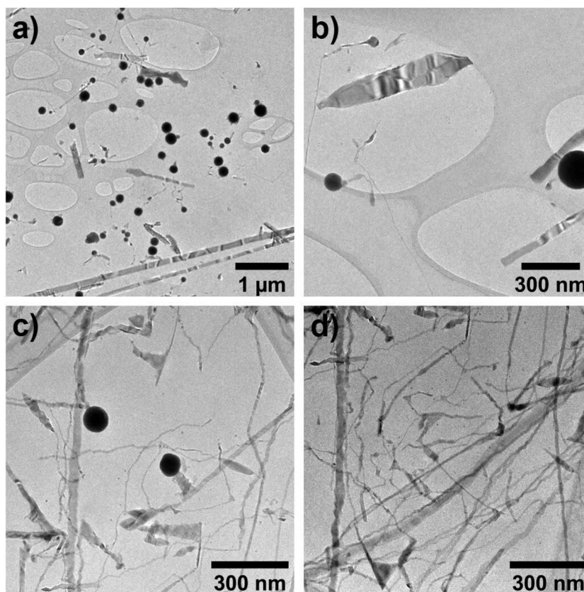
Fig. 3 TEM images of variations on the InP nanowires with 10 (a and b) or 50 (c and d) mole % extra P(NEt 3 ).
