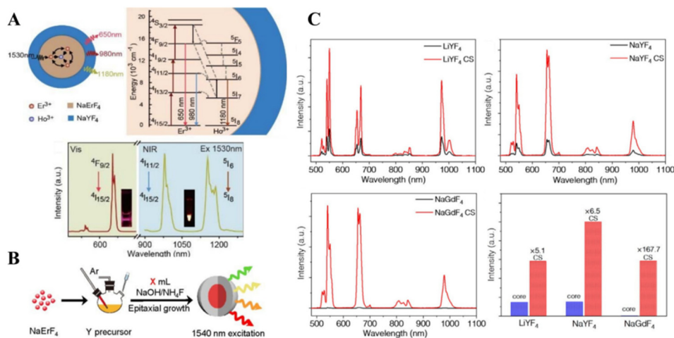
Fig. 2 (A) Energy transfer mechanism in the NaErF 4 :2%Ho@NaYF 4 core/shell UCNPs and the upconversion emission spectrum of the obtained NIR-II UCNPs. 16 (B) Schematic illustration of the synthesis of the series of core-shell upconversion nanoparticles. 17 (C) UC emission spectra of core-shell nanoparticles, and the integration of their emission peaks excited at 1532 nm. 18
