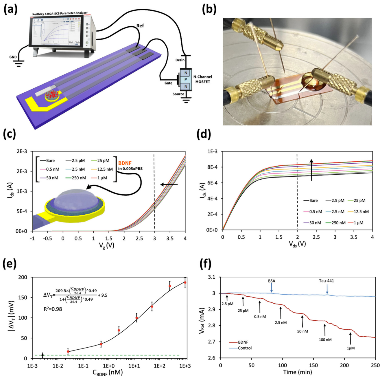
Fig. 5 (a) The schematic and (b) real image of the aptaEGFET. (c) Gate voltage–drain current ( I_{ds} – V_{gs} ) at V_D = 2 V and (d) drain voltage–drain current ( V_{ds} – I_{ds} ) at V_g = 3 V characteristics after applying different concentrations of BDNF to the r-GO/PBASE/APT/BSA modified electrode. (e) The calibration curve and LOD after adding different levels of BDNF. The baseline of the BDNF response, indicated by the green line, is characterized as the mean response augmented by a single standard deviation of three to the r-GO/PBASE/APT/BSA modified electrode of aptaEGFETs when subjected to 0.005x PBS buffer solution in the absence of BDNF. The fitted data to a Hill–Langmuir model for BDNF on the r-GO/PBASE/APT/BSA modified electrode of aptaEGFET are presented. (f) Real-time detection using an aptaEGFET for BDNF detection was investigated. BDNF was added sequentially at different levels. Control samples like BSA and Tau-441 were added at a concentration of 500 nM.
