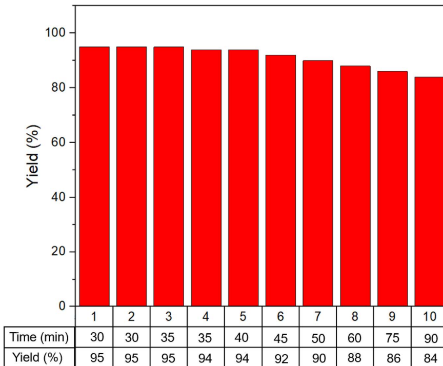
Fig. 10 Recoverability and reusability of \text{Fe}_3\text{O}_4@\text{MCM-41}@ \text{UiO-66}/\text{SB-Pd} .
