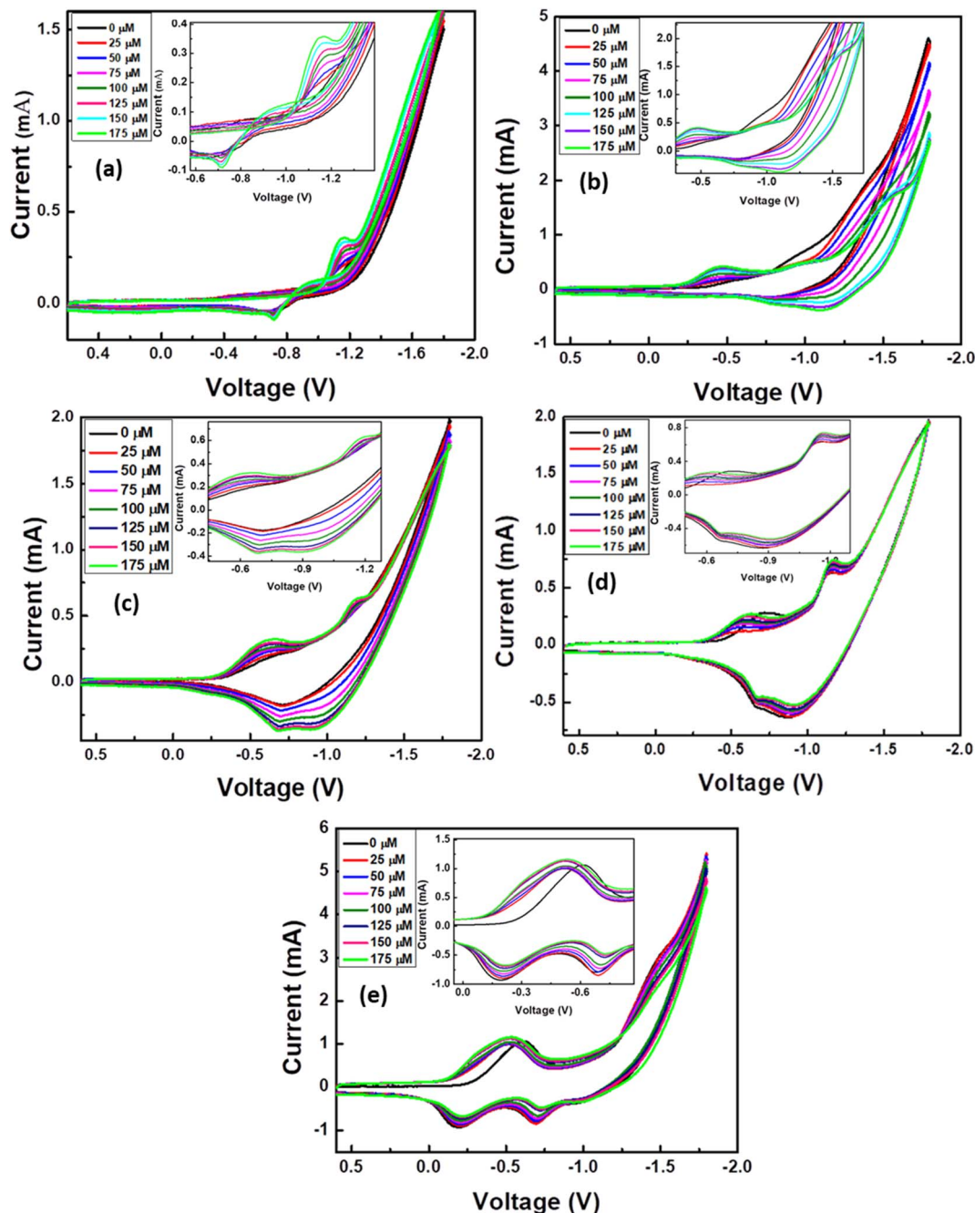
Fig. 6 Cyclic voltammogram of (a) TNP/FTO, (b) TNTs/TNPs/FTO, (c) TNTsMNG/TNPs/FTO, (d) TNTsMBU/TNPs/FTO and (e) TNTsMTU/TNPs/FTO at different concentrations of analyte. Inset shows the enlarged peak of redox species.
