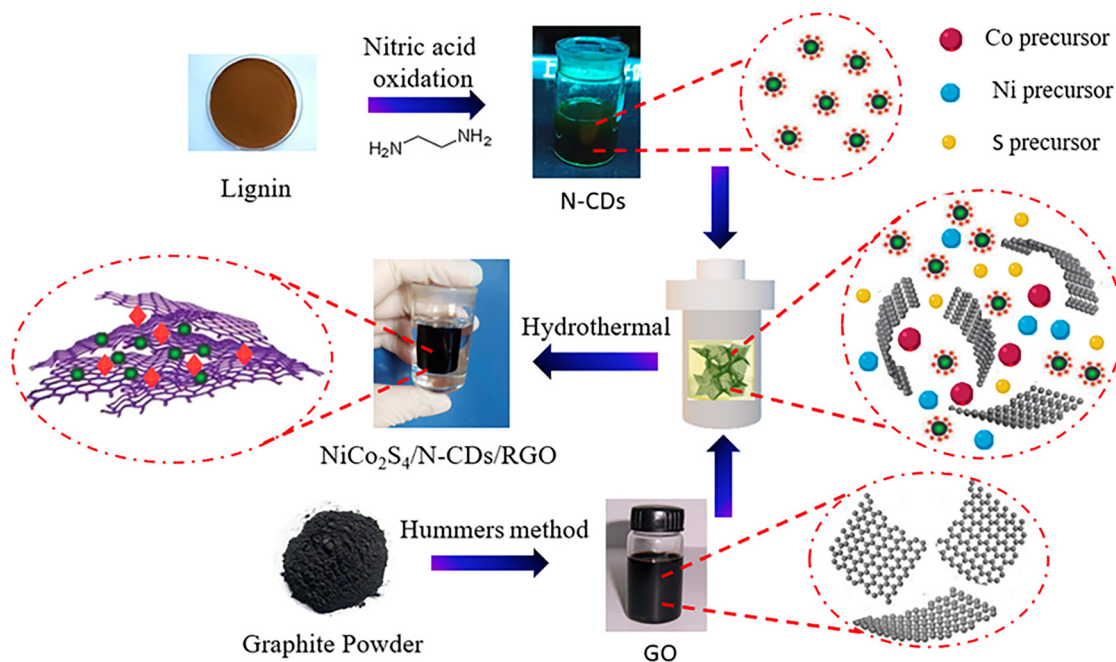
Fig. 32 Fabrication schematic of the NiCo 2 S 4 /N-CDs/RGO ternary hydrogel composite. 256 Copyright 2017, MDPI.
