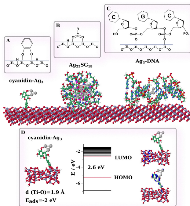
Fig. 6 Proposed anchoring modes of (A) cyanidin–Ag 3 , 105 (B) Ag 25 SG 18 , 49 and (C) Ag 3 –DNA 134 on the TiO 2 anatase model. (D) DFT optimized cyanidin–Ag 3 @TiO 2 model at PBE 135 /def2-SVP 75 level of theory as reported in ref. 105 along with corresponding energy levels and the HOMO and LUMO. Atoms are colored by element: Ag in grey, C in green, O in red, S in magenta, P in orange, N in blue, Ti in lilac and H in white.
