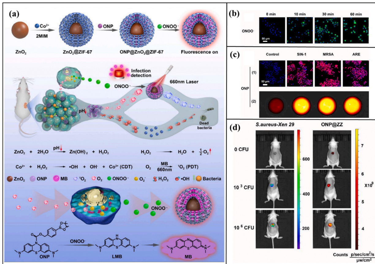
Fig. 5 (a) Preparation of \text{ONP}@ZnO_2@ZIF-67 and understanding how the nanosystem works for identifying and treating infections. (b) Macrophages expressed ONOO^- after being infected with methicillin-resistant Staphylococcus aureus (MRSA) at various time points. (c) Images of FL signals from macrophages stimulated by 3-morpholino sydnimine hydrochloride (SIN-1, ONOO^- donor), MRSA, and antibiotic-resistant Escherichia coli (ARE) were captured. (1) Seen using a confocal laser scanning microscope. (2) Viewed using an In vivo imaging system (IVIS). (d) The FL intensity of probes is used to assess the level of bacterial infection at wound locations. Reproduced from ref. 129 with permission from Elsevier, copyright 2022.
