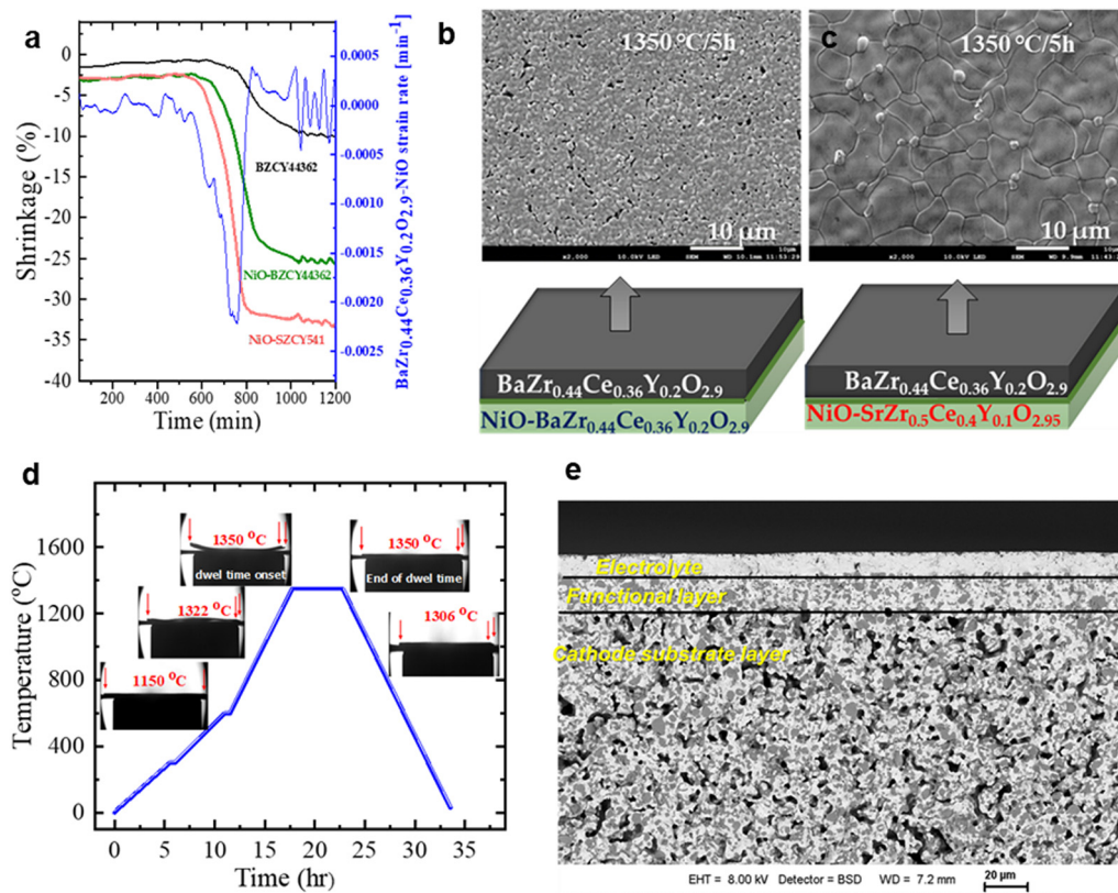
Fig. 2 (a) Shrinkage behavior of the BZCY44362 electrolyte, BZCY44362|NiO-BZCY44362 and BZCY44362|NiO-SZCY541 bi-layers determined by optical dilatometry, at a heating rate of 2^{\circ}\text{C min}^{-1} . (b) SEM image of BZCY44362 surface view on NiO-BZCY44362 electrode (c) SEM image of BZCY44362 surface view on NiO-SZCY541 after sintering at 1350^{\circ}\text{C} (d) sintering of the NiO-SZCY541 based half-cell performed under optical dilatometer, showcasing the sintering profile, and behavior of the 50 \times 50 \text{ mm}^2 size configuration with temperature and time. (e) SEM image of a polished cross-section of the fabricated half-cell.
