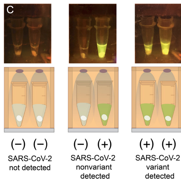
Fig. 30 Sample-to-answer device for CRISPR-based detection SARS-CoV-2 and variant nucleic acids. (A) Design of the device, including sample processing (left) and assay (right) modules. (B) Photographs of the device, which is capable of two-plex detection. (C) Smartphone-acquired fluorescence images of samples. Figure reproduced from ref. 470 under a Creative Commons CC BY 4.0 license.
