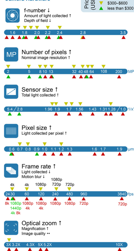
Fig. 1 Features of a modern smartphone and the potential utility of those features for developing devices for chemical and biological analysis. Aspects of the camera hardware and software-based camera control are also highlighted. The examples of hardware specifications for smartphones in three price ranges were collected from a sampling of 27 models released between 2022–2024. Specifications were from vendor websites and online consumer guides. Sensor size is expressed using the industry standard notation: a fraction of a one-inch video camera tube equivalent sensor size (i.e. 16 mm diagonal, 4 : 3 aspect ratio). A smaller value for x in 1/x'' is a larger sensor size. Pixel size was estimated from the sensor size and the total number of pixels: the dimension provided is the square root of the maximum possible area of each pixel.
