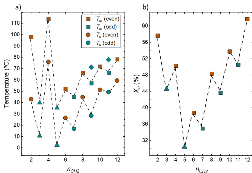
Fig. 4 (a) T_c and T_m as a function of the n_{\text{CH}_2} in the repeating unit of the \text{PE}_{n_{\text{CH}_2}} s employed. The triangles represent the data obtained by micro-DSC, while the squares and circles represent the data obtained by DSC. The rhombus symbols indicate the second melting peak in PE9 and PE11. (b) X_c variation as a function of n_{\text{CH}_2} . A color code is used to distinguish even-numbered (brown) and odd-numbered (blue) samples.
