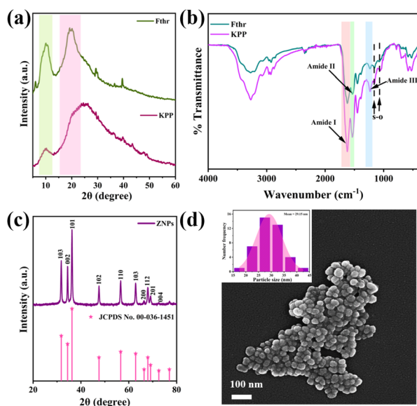
Fig. 1 (a) XRD and (b) FTIR spectra of feather microfibril (KPP) and feather (Fthr), (c) XRD spectra and (d) SEM image with inset of size distribution graph of \text{ZnO} nanoparticles (ZNPs).
