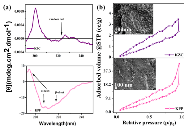
Fig. 2 (a) CD spectra and (b) BET isotherm graph of feather microfibril zinc coating material (KZC) and feather microfibril (KPP). The inset shows the SEM image before and after filling pores in KPP and KZC, respectively.
