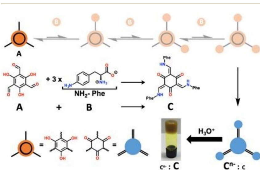
Fig. 3 A (1,3,5-triformylglucinol) and B (4-amino-L-phenylalanine) generate C^{n-} in water at pH 8, and the protonation of C^{n-} leads to the formation of a hydrogel. Reproduced from https://doi.org/10.1039/D5FD00016E with permission from the Royal Society of Chemistry, licensed under CC BY 3.0.
