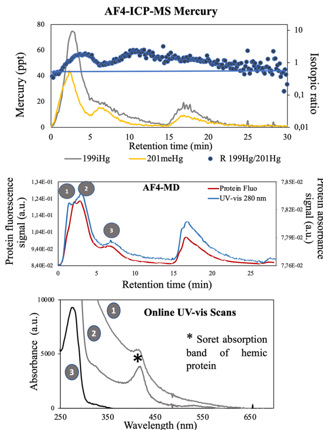
Fig. 5 Size-resolved analysis of simultaneous mercury ( 199 iHg) and methyl-mercury ( 202 MeHg) interactions with EPS components released by a diatom, C. meneghiniana , (A) and a cyanobacterium, Synechocystis sp., (B) using AF4-ICP-MS and UV-Fluo. The isotopic ratio is present as the log of ( 199 iHg/ 201 MeHg). The ratio increased as iHg bound to EPS increased compared with MeHg (>1), but decreased when MeHg bound to EPS increased compared with iHg (<1). The UV-vis scans, obtained at different retention times with AF4-MD (labelled 1, 2 and 3) are presented, allowing the identification of hemic protein with Soret absorption band (*) eluting mainly at retention time 2. Fractionation conditions and settings are provided in ESI † section S4 (unpublished data).
