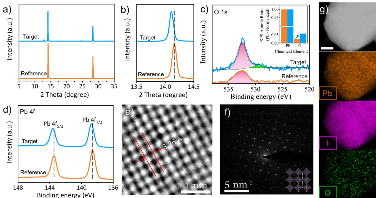
Fig. 2 (a) XRD patterns, (b) XRD patterns from 13.5 to 14.5^\circ , (c) HR XPS O 1s spectra (inset shows the atomic ratio of oxygen normalized to lead (Pb 4f) peak intensity) and (d) XPS Pb 4f spectra of the reference and target perovskite films. (e) HRTEM image, (f) SAED pattern, (g) HAADF-STEM (scale bar: 200 \text{ nm} ), and the corresponding elemental mapping images of the target perovskite film.
