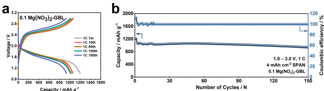
Fig. 6 Full battery tests using 0.1 \text{Mg}(\text{NO}_3)_2 -GBL electrolyte. (a) Voltage hysteresis of Li/SPAN batteries with 0.1 \text{Mg}(\text{NO}_3)_2 -GBL electrolyte in the voltage range of 1.0–3.0 V. Sulfur loading in the SPAN cathode is 4 \text{ mA h cm}^{-2} . (b) Cyclic stability of full cell for cycling at 1 C.
