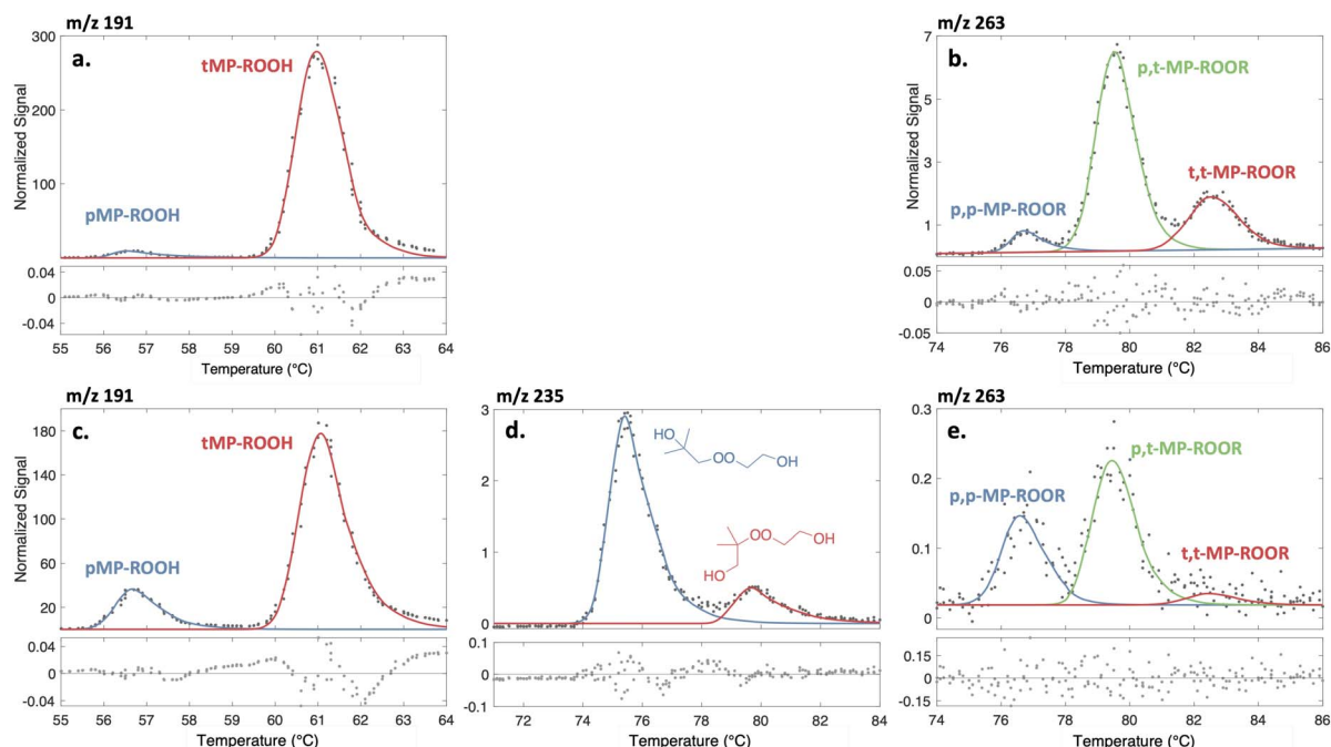
Fig. 1 Representative chromatograms of ROOH (a and c) and ROOR (b, d, and e) products formed in the oxidation of 2-methylpropene in experiments with high RO_2/HO_2 ratios (top row) and high HO_2/RO_2 ratios (bottom row). Experiments represented in the bottom row also included ethene. The experimentally measured signal is given as dark gray dots, while the colored lines are the bootstrap best fits of the chromatographic data. The corresponding structures are the assignments of these peaks. Below each chromatogram are plots of the residuals of the best fits given as fractions of the maximum peak value.
