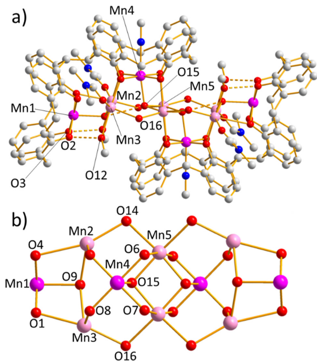
Fig. 4 (a) Molecular structure of complex 3 . (b) Metal–oxygen core of 3 . Colour code: Mn III = magenta, Mn II = pink, O = red, N = blue, C = grey. H atoms, t Bu groups, some endo-cavity solvent, and solvent of crystallisation omitted for clarity.
