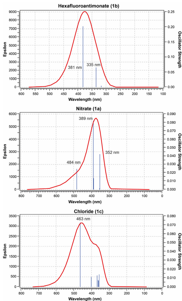
Fig. 9 Theoretically predicted (TPSSh) UV/Vis absorption spectra of 1b , 1a , and 1c (with R = n Bu and SbF 6 - , NO 3 - , or Cl - counterions, respectively).
