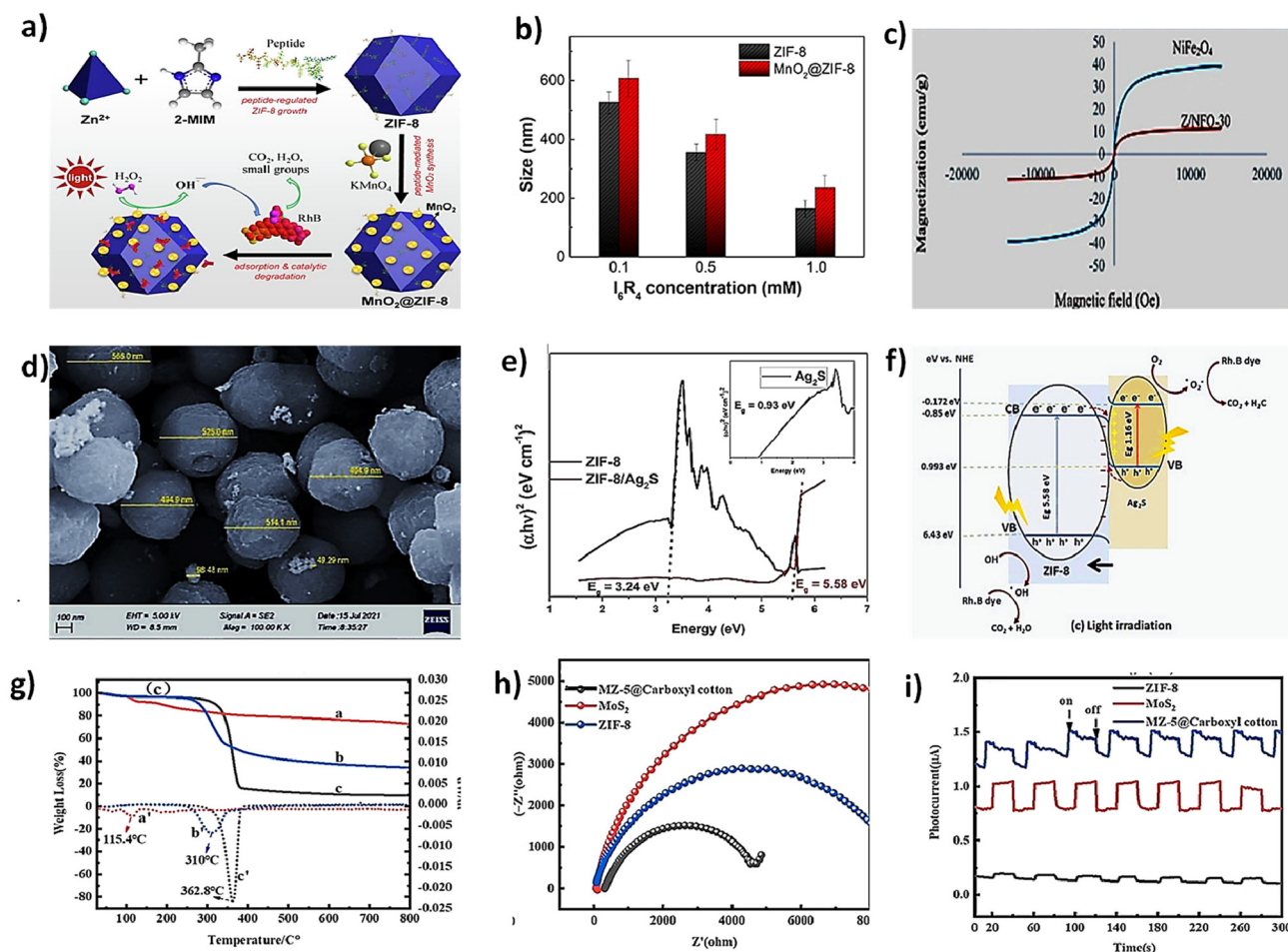
Fig. 6 (a) Fabrication of \text{MnO}_2 @ZIF-8 core-shell nanocomposites. (b) Size (hydrodiameter) distribution of the ZIF-8 crystals and the \text{MnO}_2 @ZIF-8 nanocomposites prepared at varied peptide concentrations [reproduced from ref. 170 with the permission from Elsevier, copyright 2021]. (c) Magnetic hysteresis curve of \text{NiFe}_2\text{O}_4 nanoparticles and Z/NFO-30 composite [reproduced from ref. 92 with the permission from Elsevier, copyright 2020]. (d) FE-SEM of ZIF-8/ \text{Ag}_2\text{S} . (e) Optical bandgap for ZIF-8, \text{Ag}_2\text{S} , and ZIF-8/ \text{Ag}_2\text{S} by using Tauc plots. (f) S-scheme mechanism of ZIF-8/ \text{Ag}_2\text{S} photocatalyst under vis-light irradiation [reproduced from ref. 180 with the permission from Elsevier, copyright 2016]. (g) TG and DTG curves of \text{MoS}_2 /ZIF-8 composite (a and a'); MZ-5@Carboxyl cotton (b and b'); pristine cotton fabric (c and c'). (h) EIS plots of MZ-5@Carboxyl cotton, \text{MoS}_2 and ZIF-8 (i) transient photocurrent responses of \text{MoS}_2 , ZIF-8 and MZ-5@Carboxyl cotton [reproduced from ref. 189 with the permission from Elsevier, copyright 2016].
