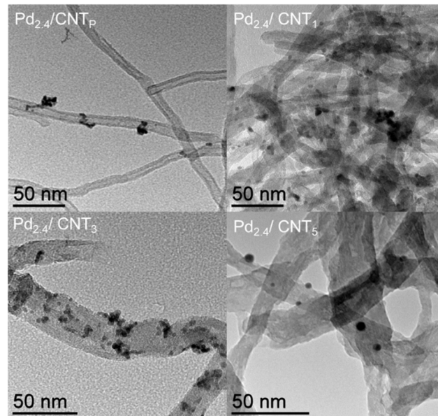
Fig. 3 TEM images of the CNT-supported Pd 2.4 nanoparticles.
