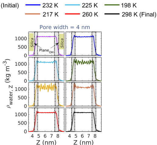
Fig. 8 Mass density of water ( \rho_{\text{water},z} ) as a function of the distance along z axis of the simulation cell for slit pore of width 4 nm at the control temperatures as used in the simulations. The slit pore being symmetric, the arrows indicate the width of the (interface + shell) layer of confined water in contact with the amorphous silica surfaces. The first and fourth dash-dotted lines in each profile represent the z index of the geometric center of the hydroxyl groups on the silica surface exposed to the water medium that essentially lies on the plane of the hydroxyl groups, whereas the second and third dash-dotted lines indicate the boundaries of the (interface + shell) layer formed by confined water. The average width of the (interface + shell) layer of water in different slit pores is provided in Table 2(3). The profiles for 6 and 8 nm pores are provided in Fig. S5.
