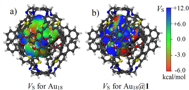
Fig. 2 The electrostatic potential surface for the isolated Au 18 cluster (a) and overall Au 18 @1 (b) aggregate drawn at a 0.001 electrons per Bohr 3 electron density for the Au 18 cluster (including the 1 host structure for graphical guidance). Blue denotes electro-positive sites prone to interact with Lewis bases.
