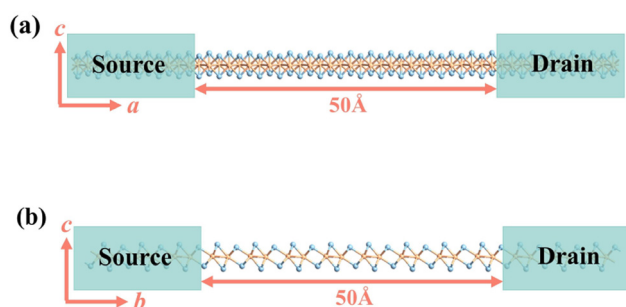
Fig. 3 Schematic diagrams of the two-probe system for computing the electric transport of monolayer O1 variant of ZrCl 2 in (a) the a direction and (b) the b direction. The channel length is 50 Å.
