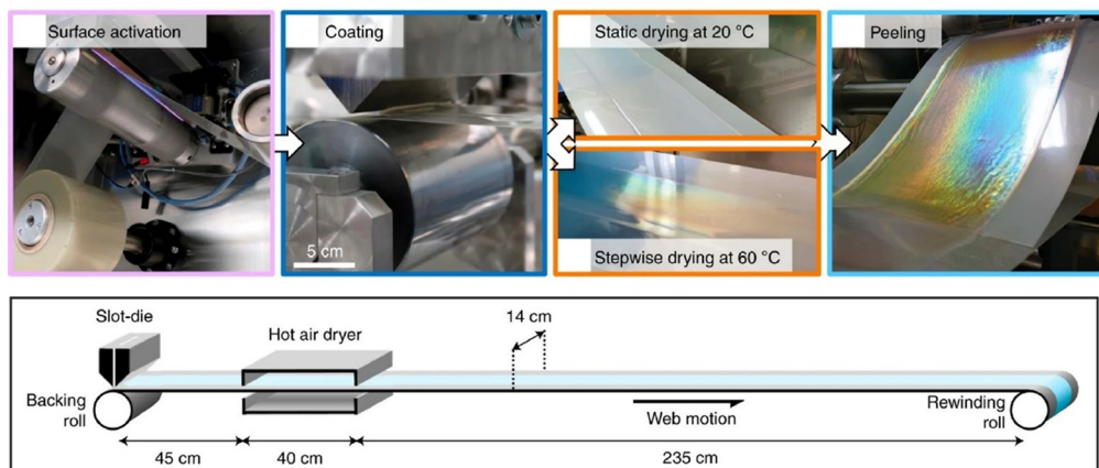
Fig. 11 Large-scale production of structurally coloured cellulose nanocrystal films using roll-to-roll deposition: flow chart (top), process photos (middle), and schematic of the pathway (bottom). Reprinted with permission from ref. 54 copyright 2021 Springer-Nature.
