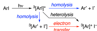
Scheme 1 Aryl iodide photolysis leading to radical and triplet aryl cation intermediates.
