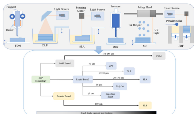
3DP techniques nomenclature: FDM: Fused deposition modelling; SLA: Stereolithography apparatus; DLP: Digital light processing; 2PP: two-photon polymerization; SLS: Selective laser sintering; MJ: Material jetting; PBF: Powder bed fusion
