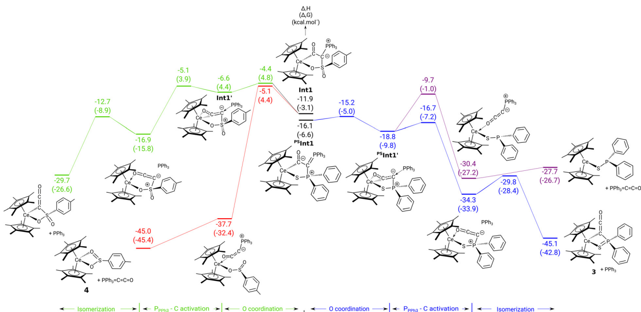
Fig. 3 Computed enthalpy (kcal mol -1 ) profile for the transformation of complex 1 to 3 (right) and 2 to 4 (left) upon CO addition.
